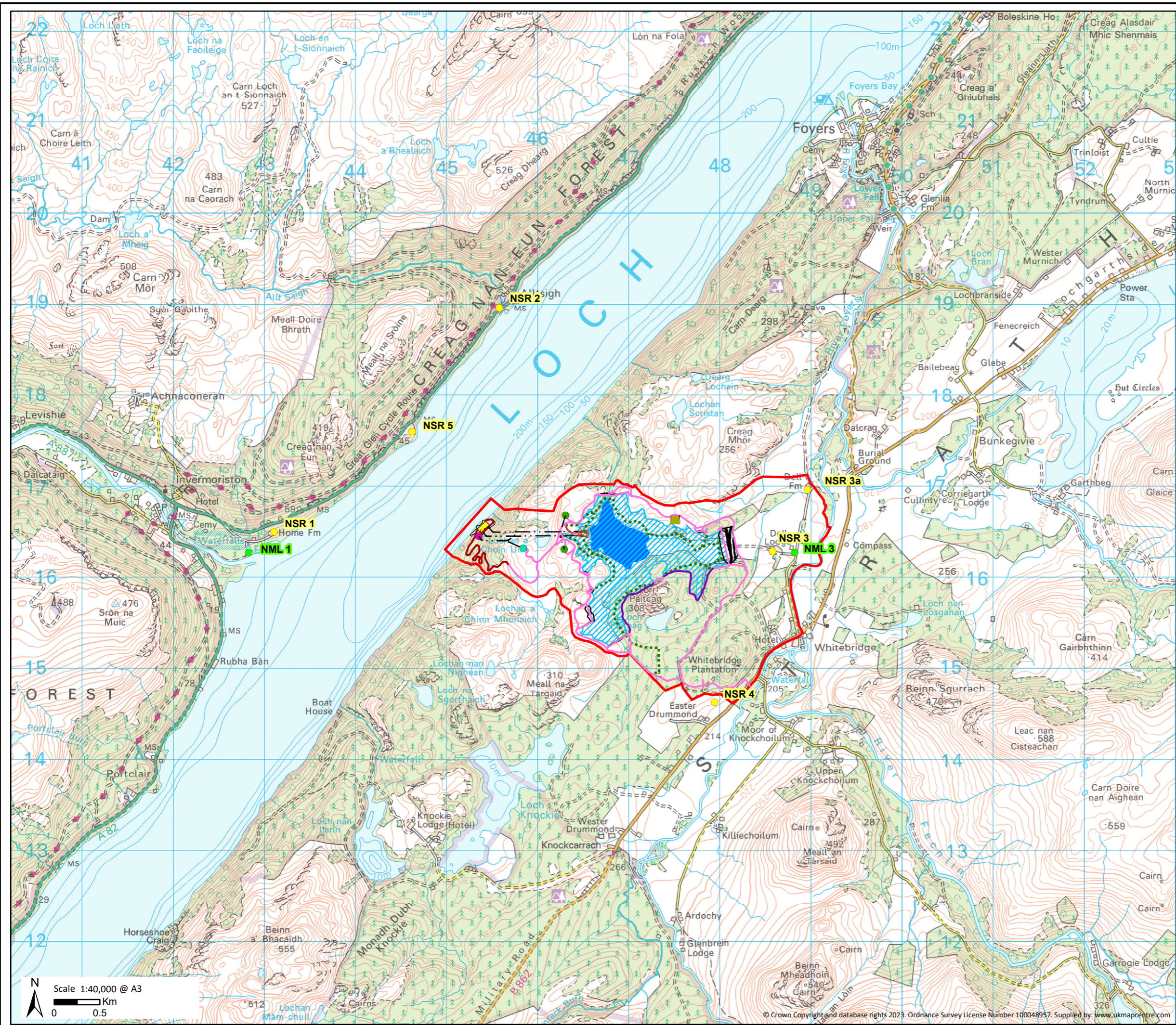
Figure 17.1 Noise Sensitive Receptors (NSRs) and Noise Monitoring Locations (NMLs)
